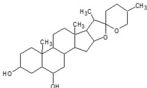
(3b, 5a, 6a, 25R)- Spirostan-3, 6-diol
